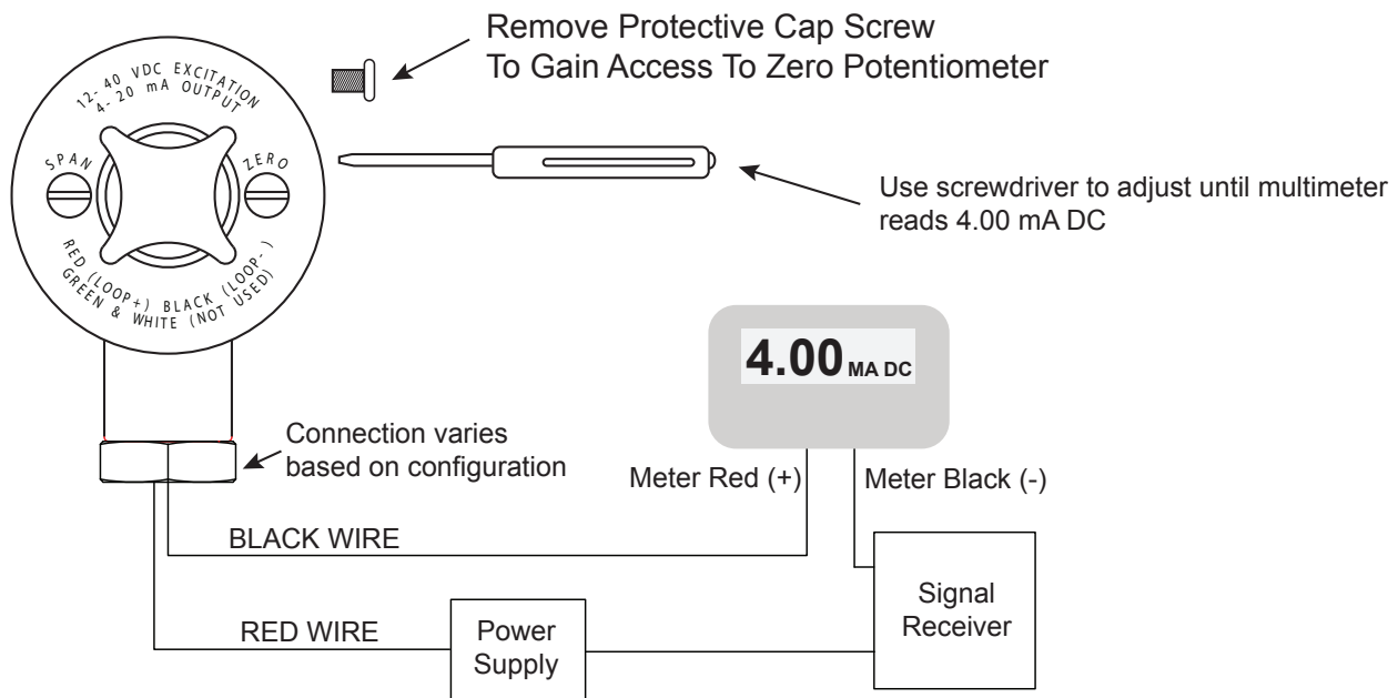
Figure 3 Zero Adjustments
