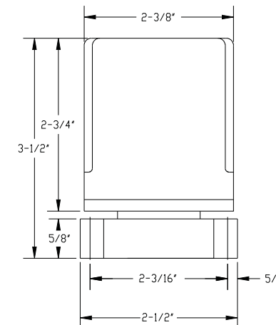
Relay Type 3 Dimensions
