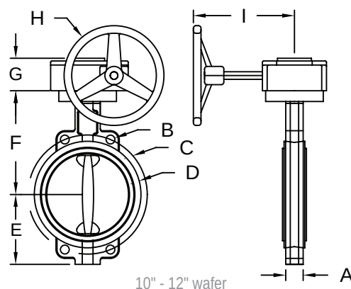
10" - 12" wafer
