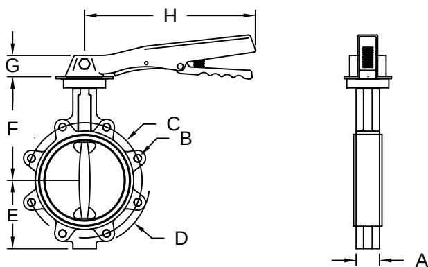
2" - 8" wafer
