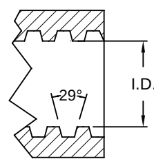
female thread
