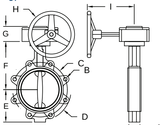
10" - 12" wafer
