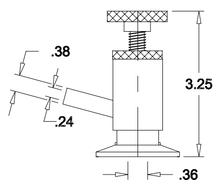
CLAMP STYLE
