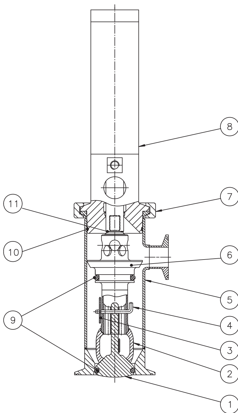
Cross Sectional Drawing Toftejorg SaniMidget Retractor, Pneumatic Driven Art. nos. TE75M100_132
