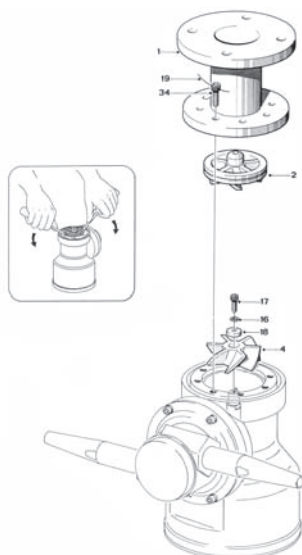
Top assembly
