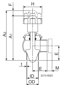
Figure 4. Dimensions
